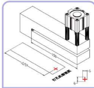
"+"6*6mm Breathing hole
