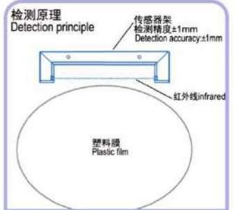
吹膜机宽度检测仪 Film blowing machine width detector
